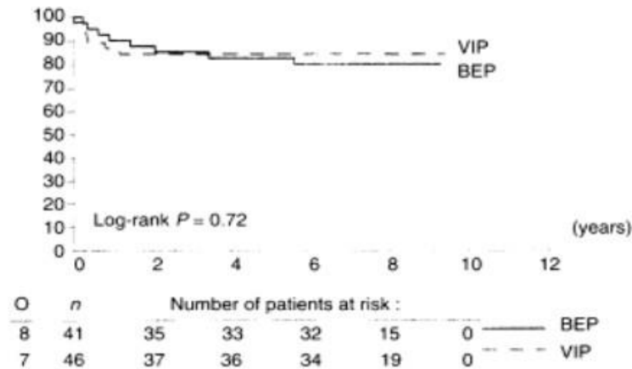
Figure 1 Progression-free survival
